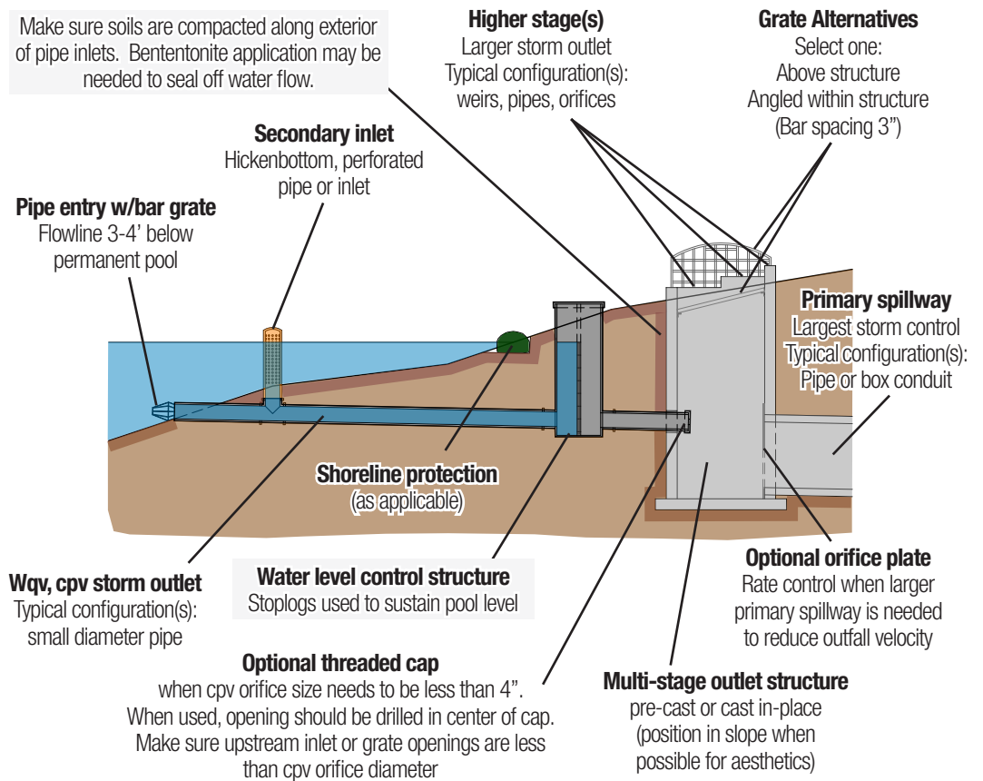
Figure 9.11-1-11: Multi-Stage Outfall Structure Example Elements
